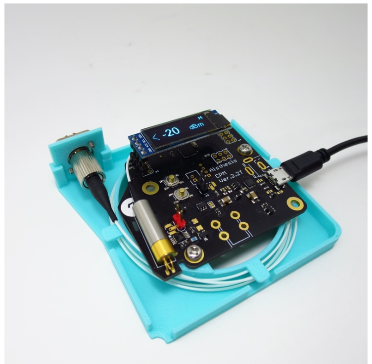
Compact Optical Power Monitor Board
